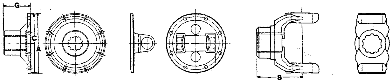
COMPANION FLANGE
