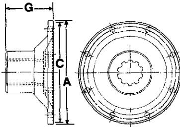
COMPANION FLANGE
