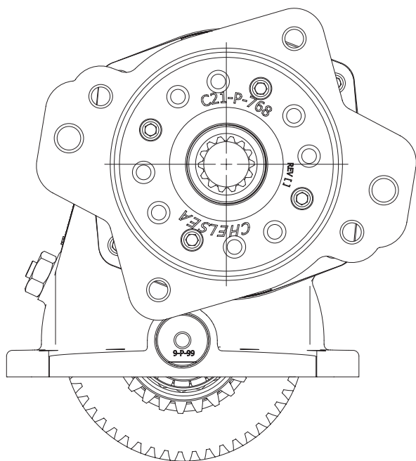
3 Arrangement
