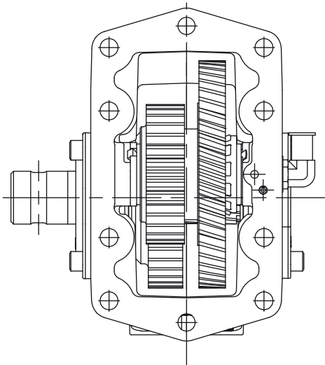
Assembly 5
