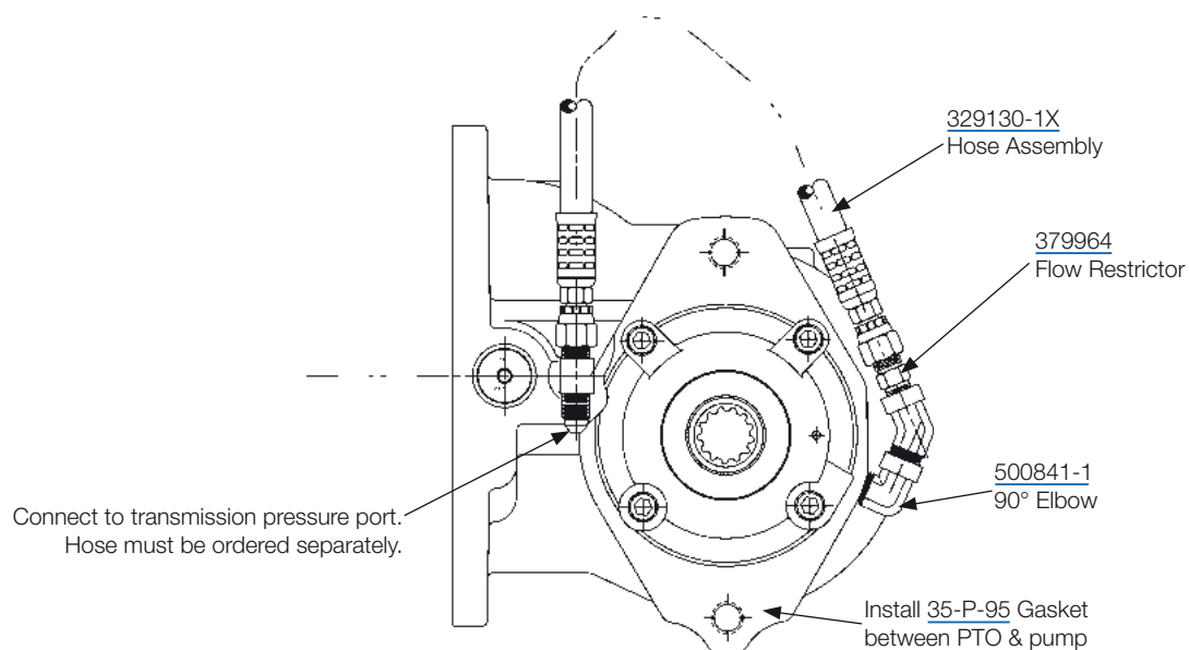
Assembly View 3
