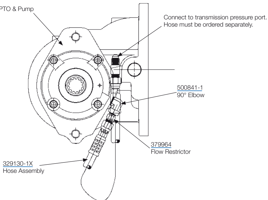
Assembly View 5
