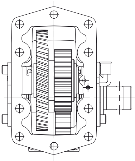
Assembly 3
