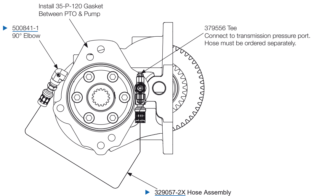
Assembly View 5
