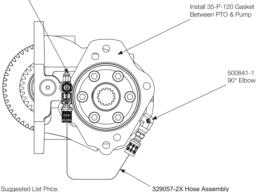
Assembly View 3
