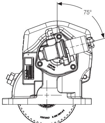
5 Arrangement
