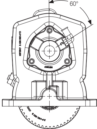
8 Arrangement
