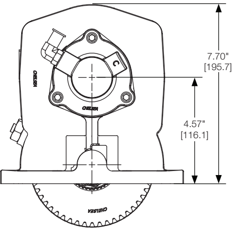
Assembly 8
