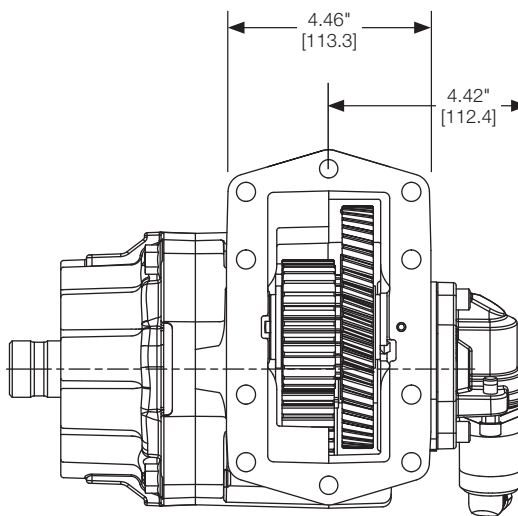
Assembly 5
