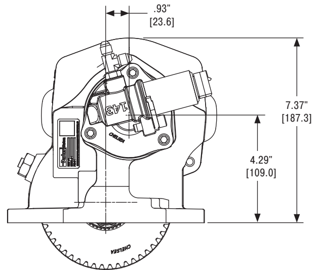
Assembly 5
