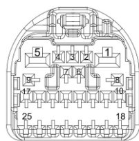
CONNECT REAR VIEW (WIRE SIDE)
