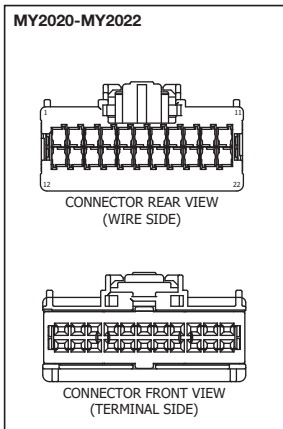
Ford Interface Connector Detail Male Connector (Shown) Provided with Vehicle
