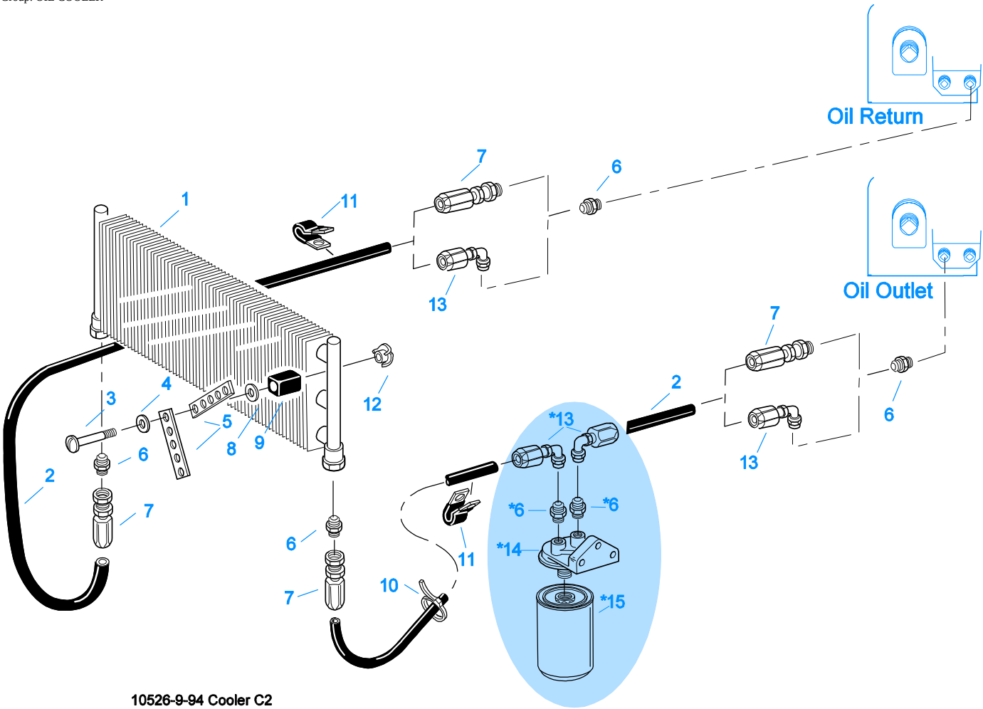
10526-9-94 Cooler C2
