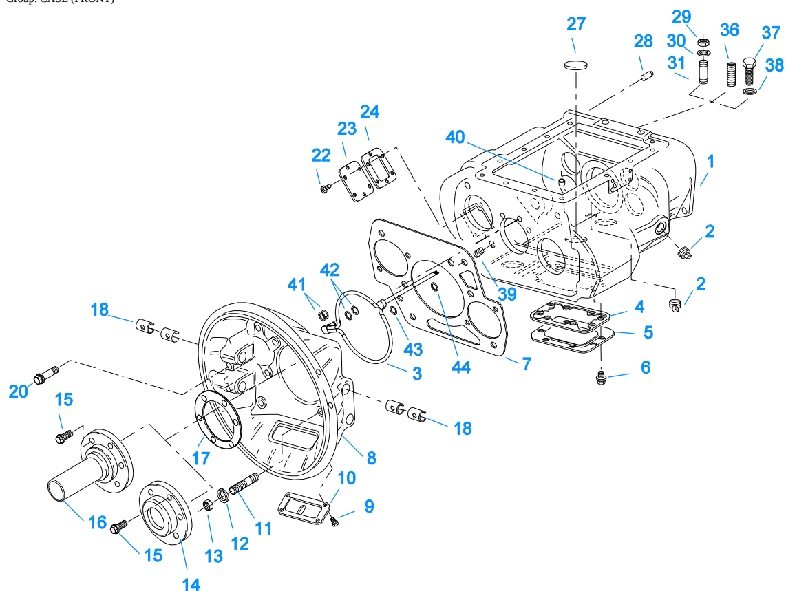
10319-11-99 Alum Hsg
