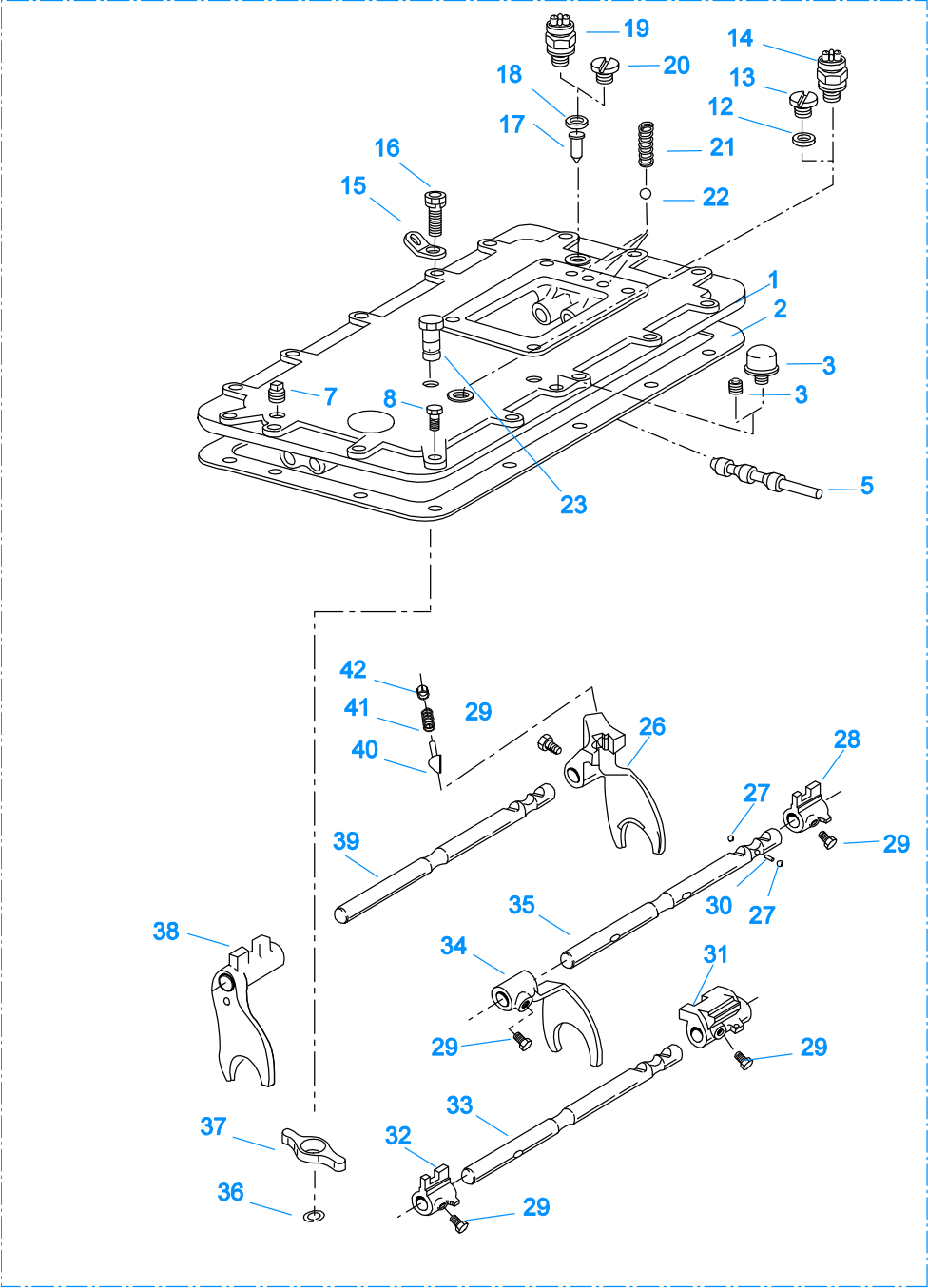
10245-1-01 X-Bar
