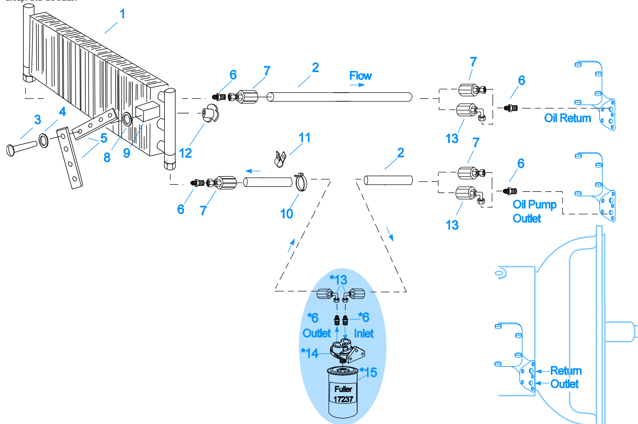
10525-4/92 Cooler
