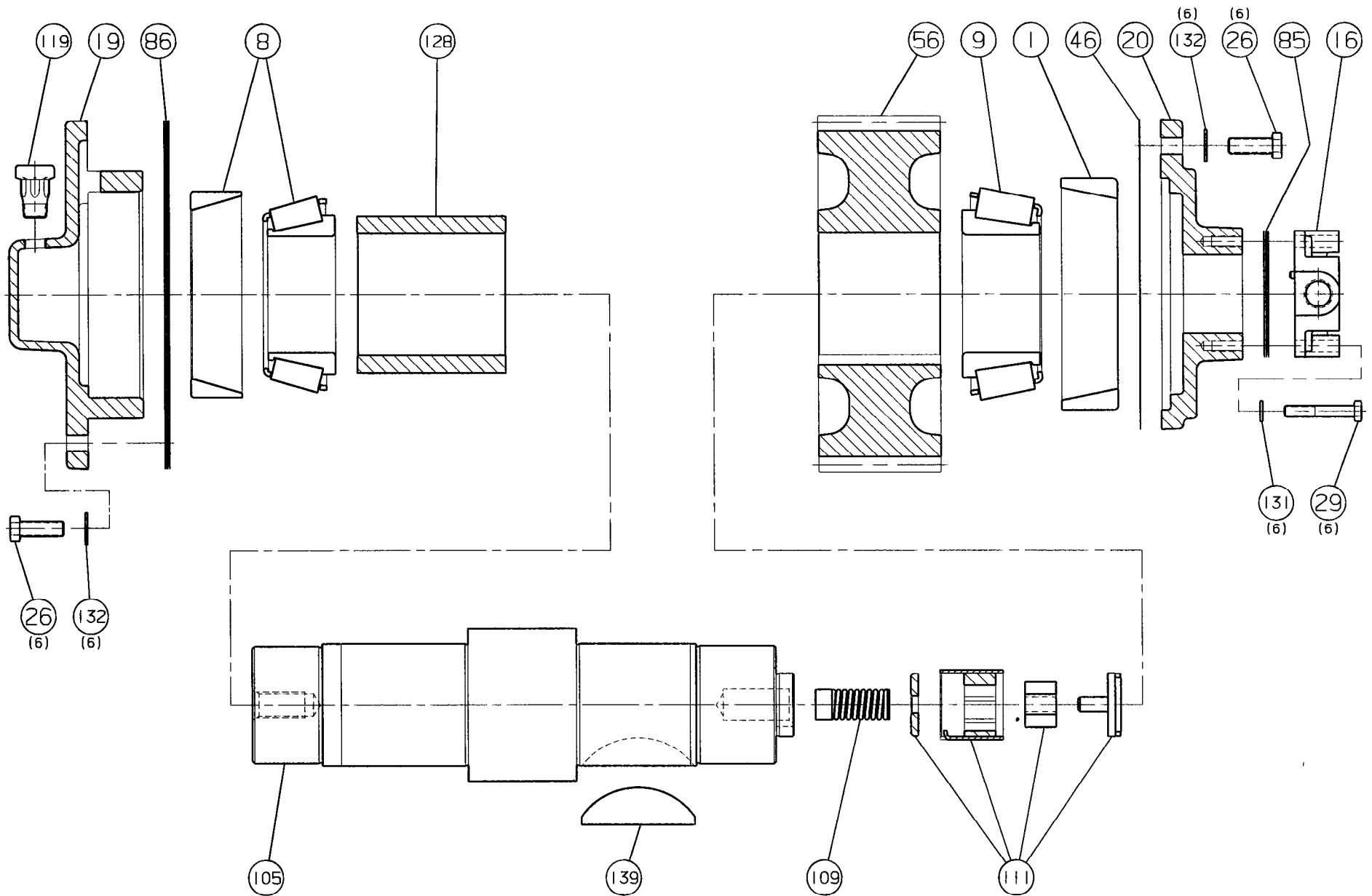
FIGURE 8.3 TC-1421 INTERMEDIATE SHAFT PARTS
