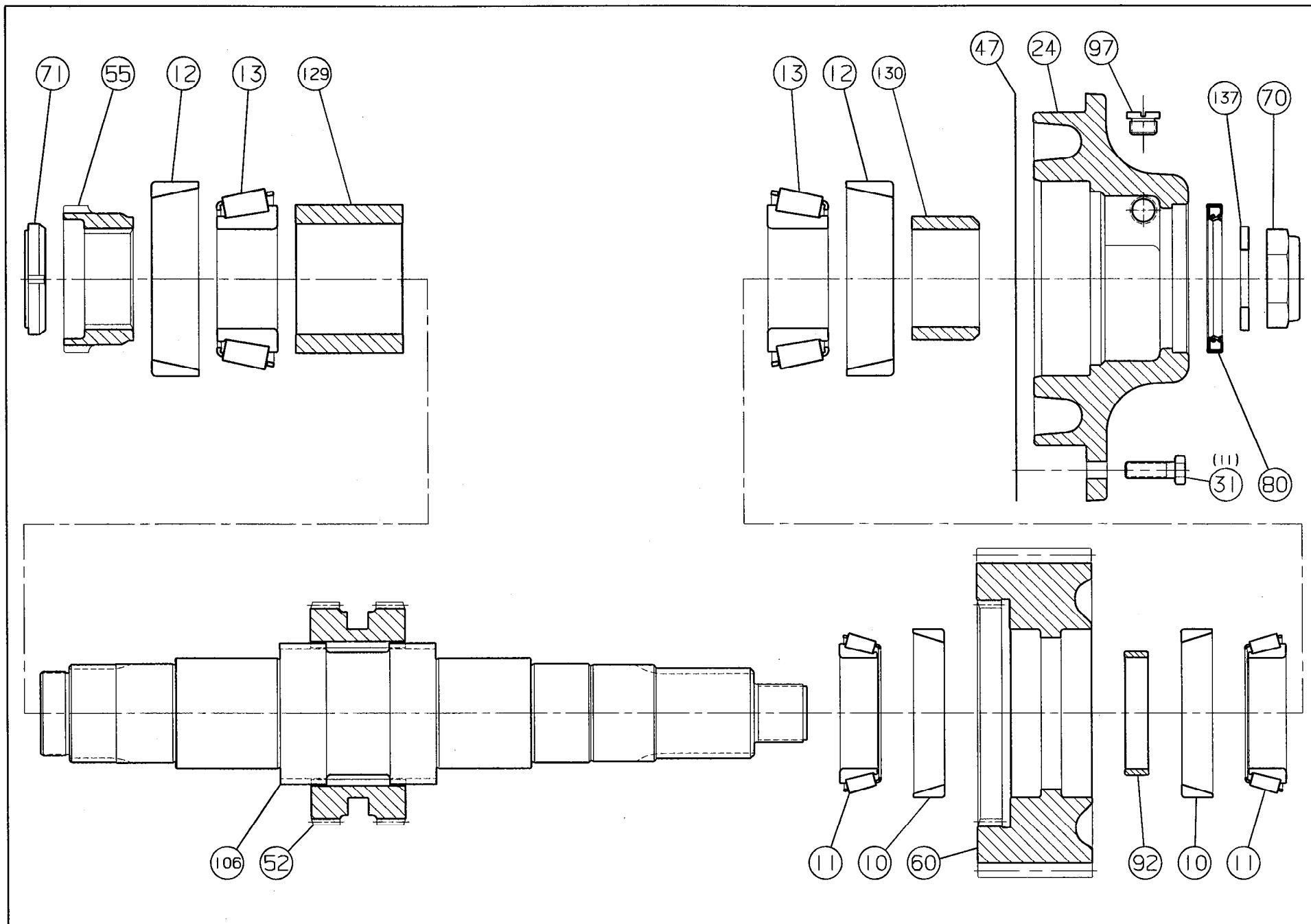
FIGURE 8.5 TC-1421 LOWER SHAFT PARTS
