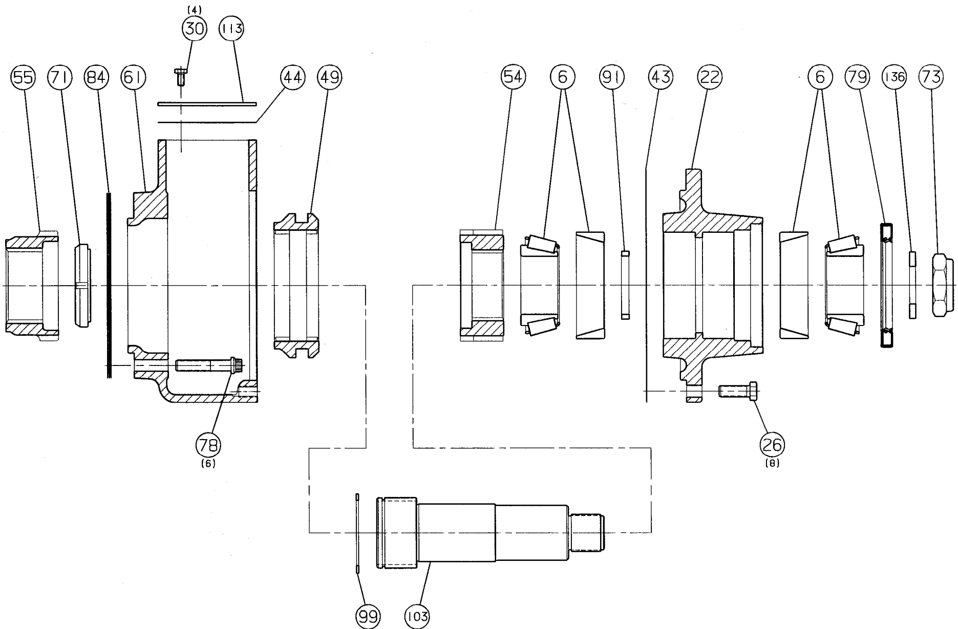
FIGURE 8.7 TC-142 & TC-1421 PTO OUTPUT SHAFT PARTS
