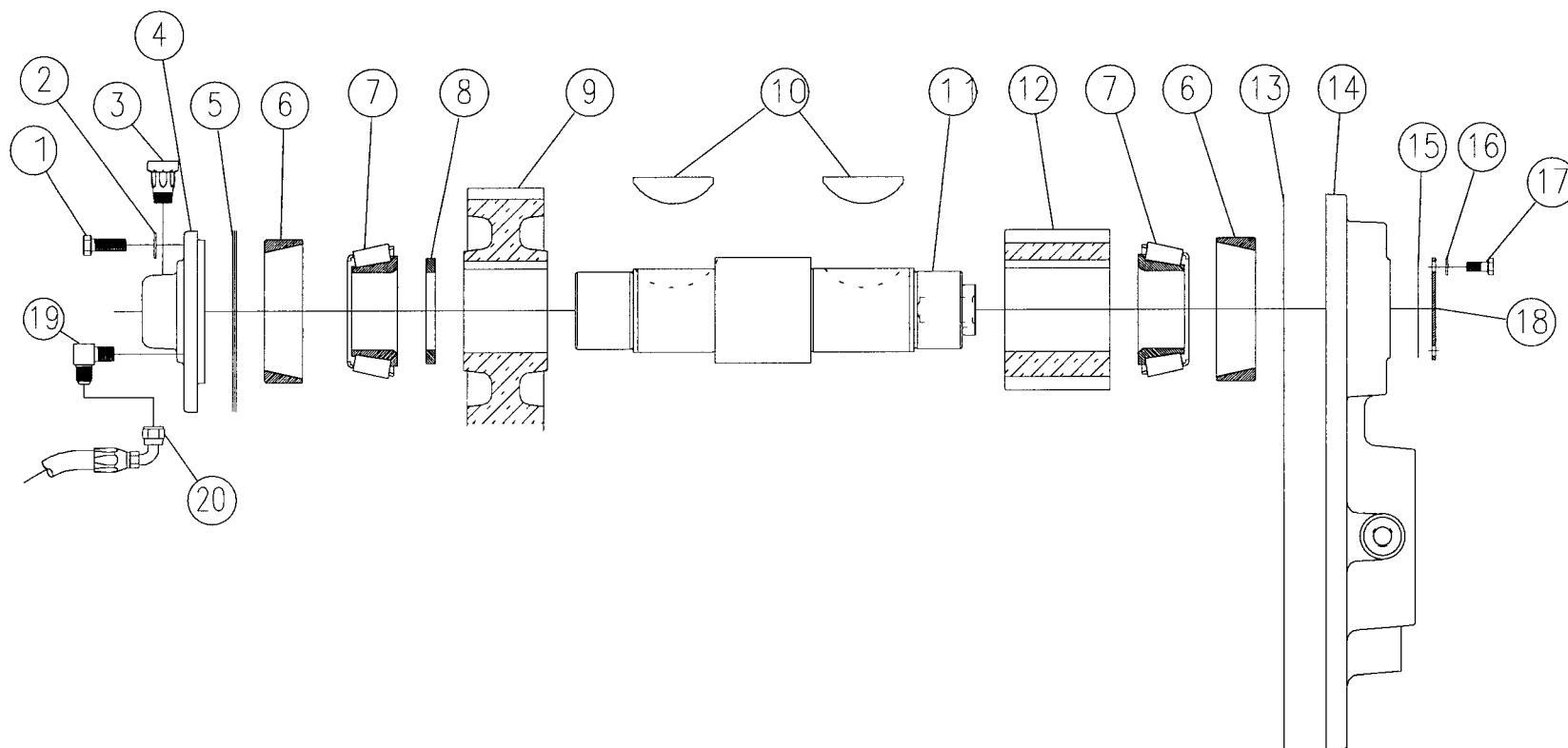
TC-270 INTERMEDIATE SHAFT ASSEMBLY WITHOUT LUBRICATION
