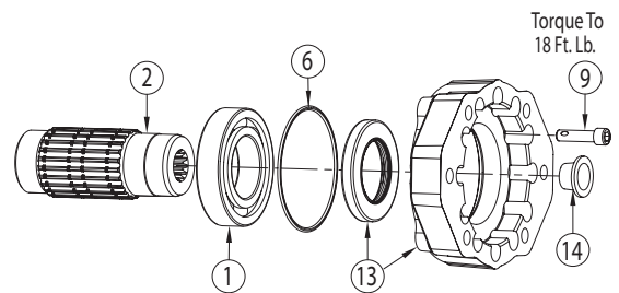
CD05/10 – “2” & “C” Output Option
