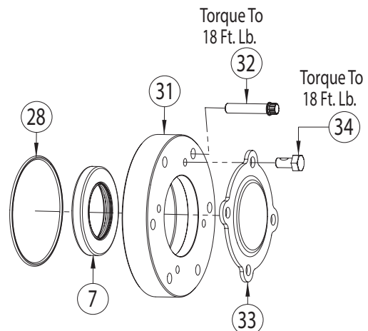
CD10 – Greaseable Bearing Cover Assembly
