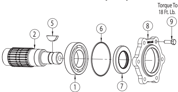
CD05/10 – “B” Output Option
