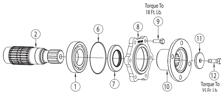
CD05/10 – “2” & “C” Output Option
