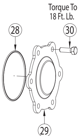
CD05/10 – Bearing Cover Assembly
