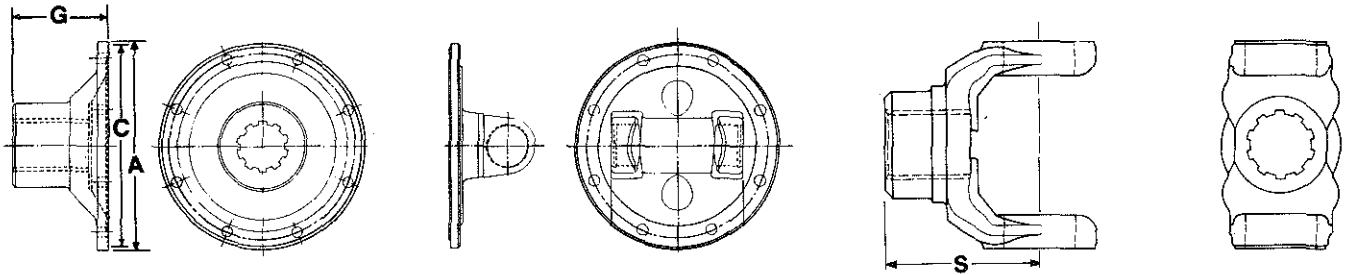
COMPANION FLANGE
