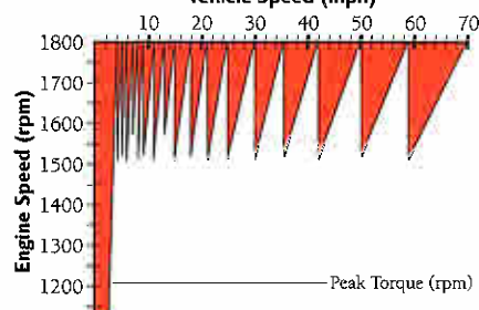
18-SPEED PERFORMANCE CHART Vehicle Speed (mph)
