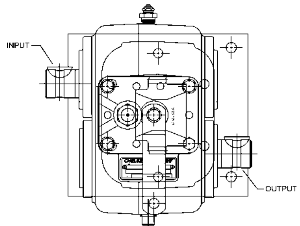
Ass'y H
